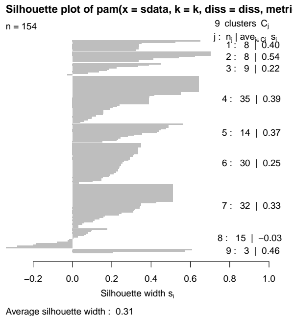
Figure 10.4: Clusters of Tweets
