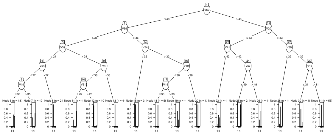
Figure 8.9: Decision Tree
