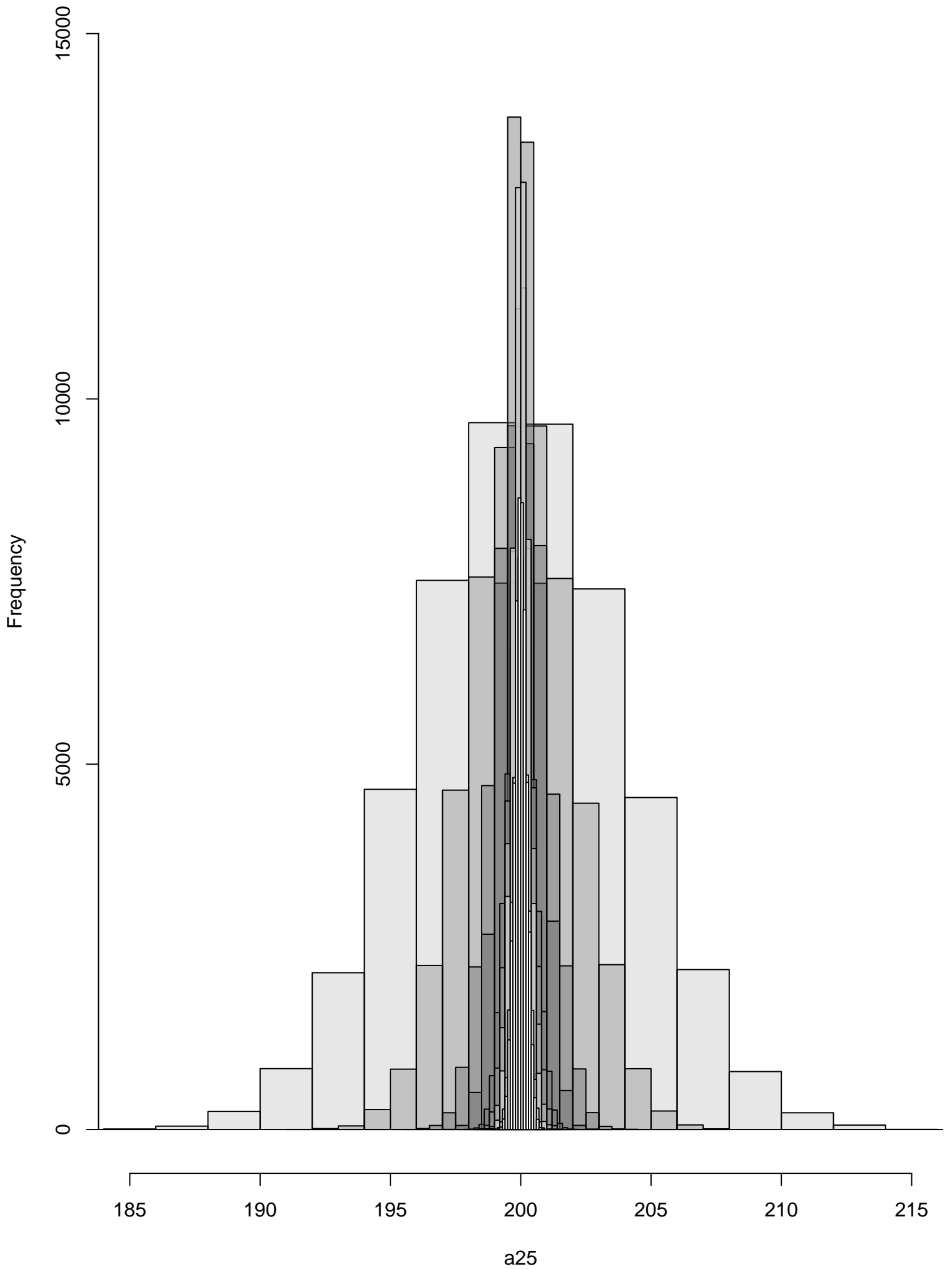
Histogram of a25
